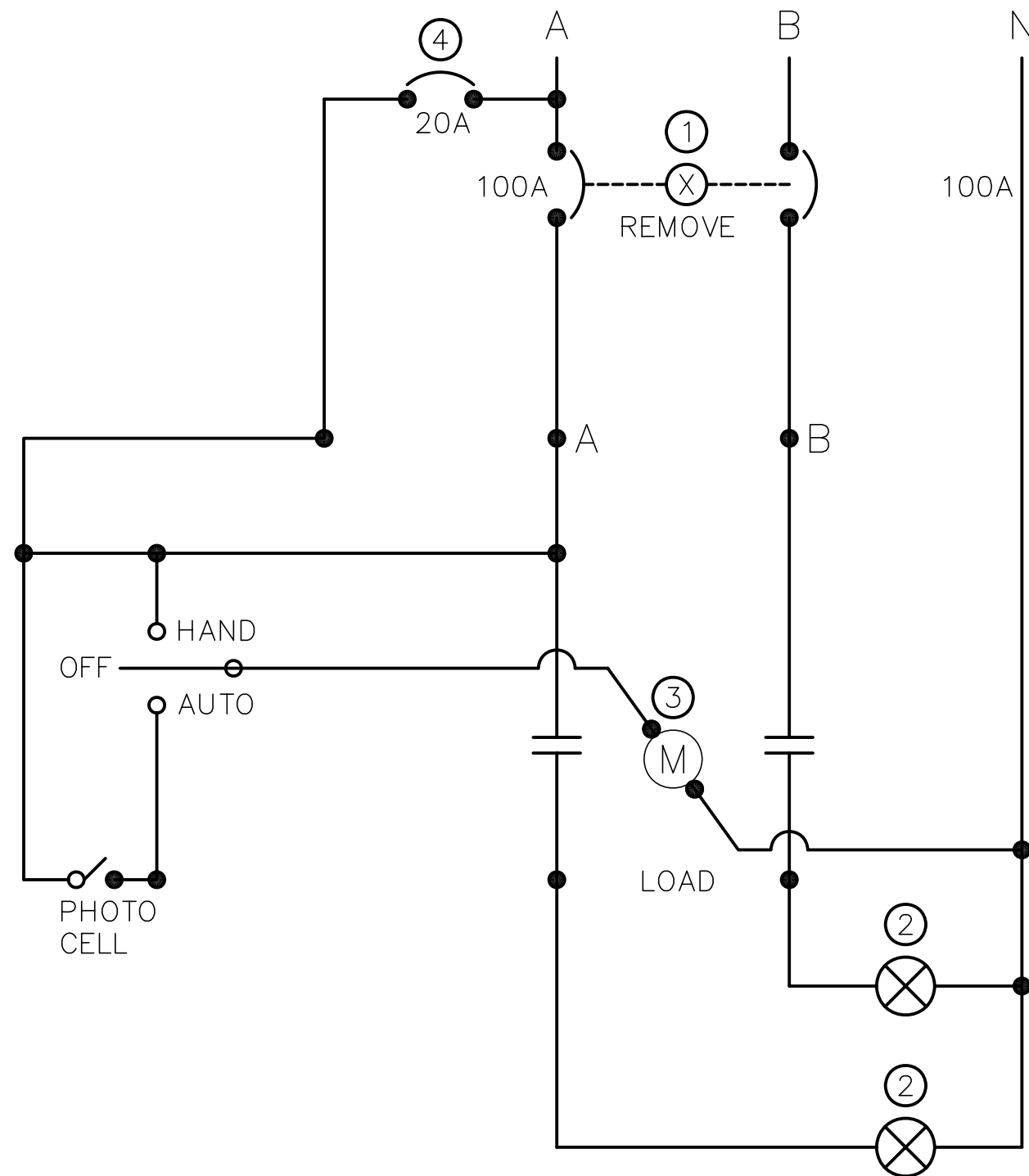
LIGHTING CONTRACTOR WIRING DIAGRAM (120 V COIL)
