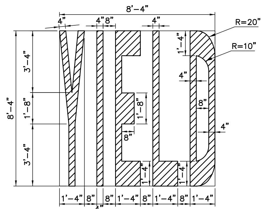
WORD MARKING DETAIL NOT TO SCALE
