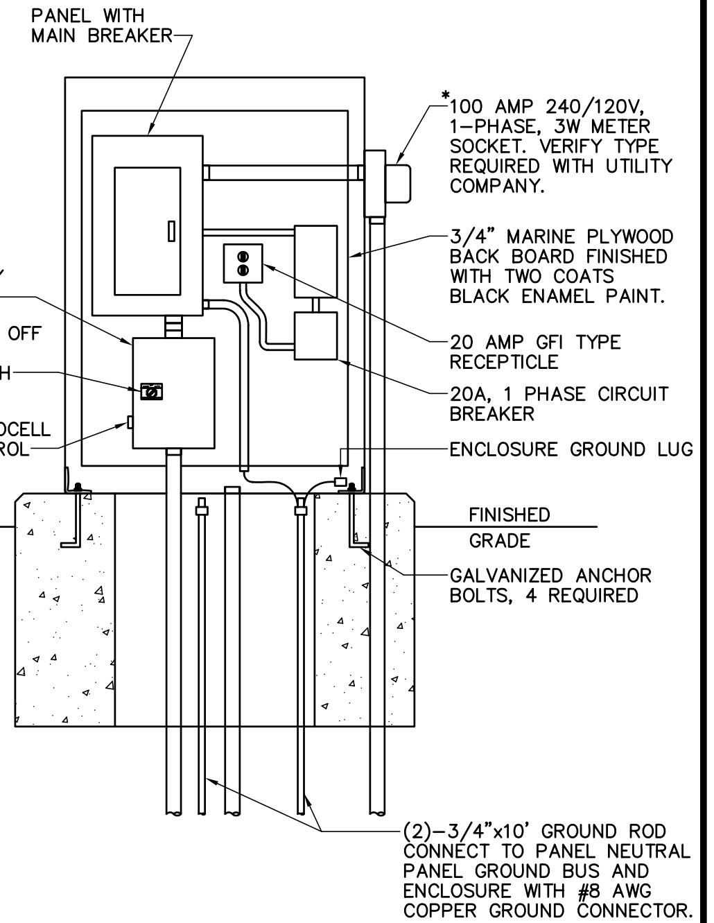
INTERIOR ELEVATION
