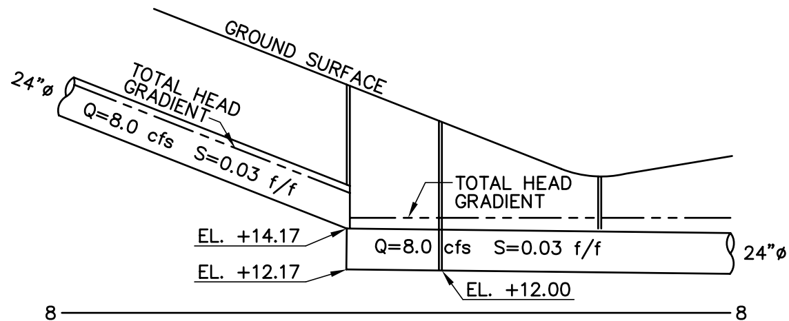
CASE NO. 2 - DROP MANHOLE, NO IMPACT
