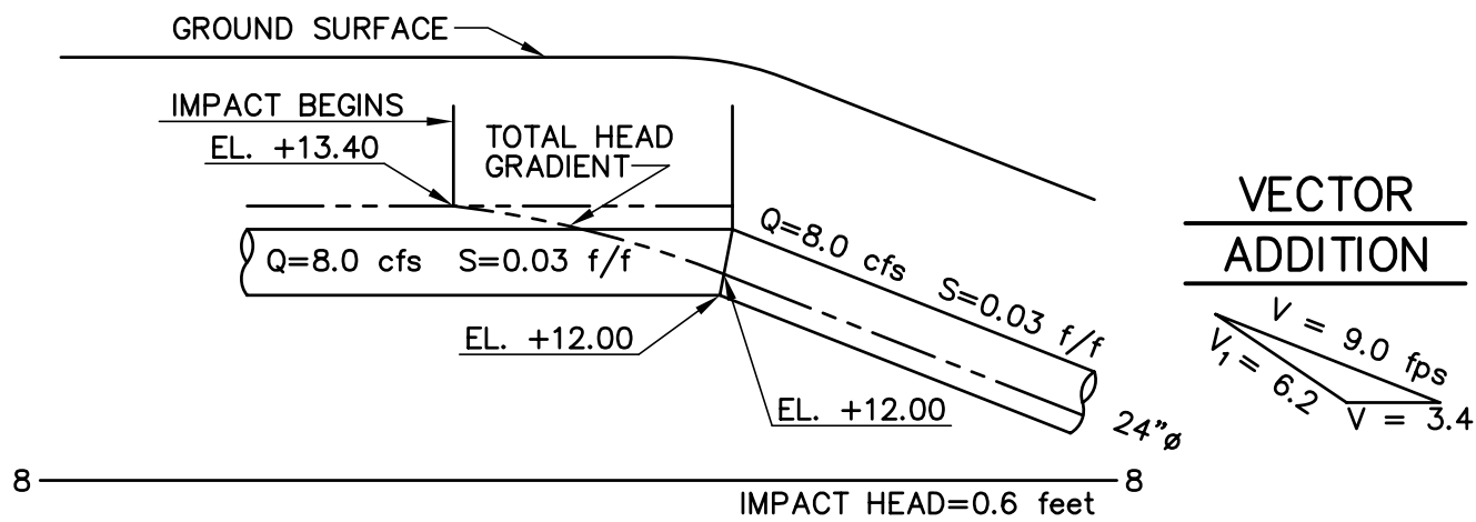
CASE NO. 3 - IMPACT IN DOWNSTREAM PIPE
