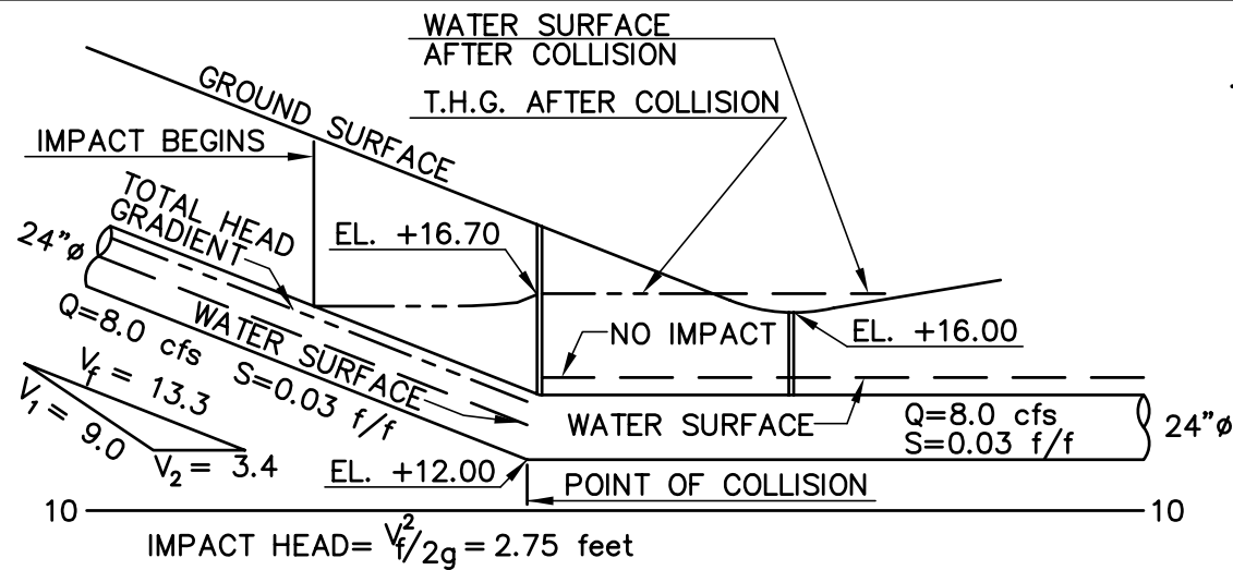
CASE NO. 1 - IMPACT IN UPSTREAM PIPE
